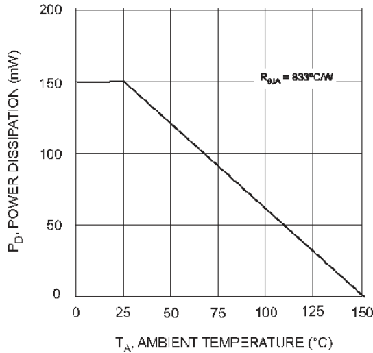
Fig. 1 Derating Curve
